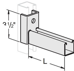
CLEVIS BRACKET OPENING UP
