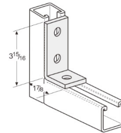
3 HOLE CORNER ANGLE L1113
