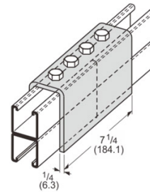
4 HOLE SPLICE CHANNEL L1308
